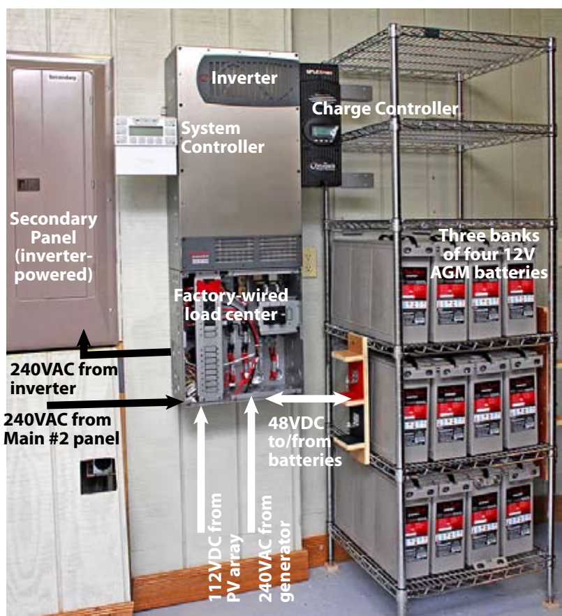
Electrical connections inside equipment room
